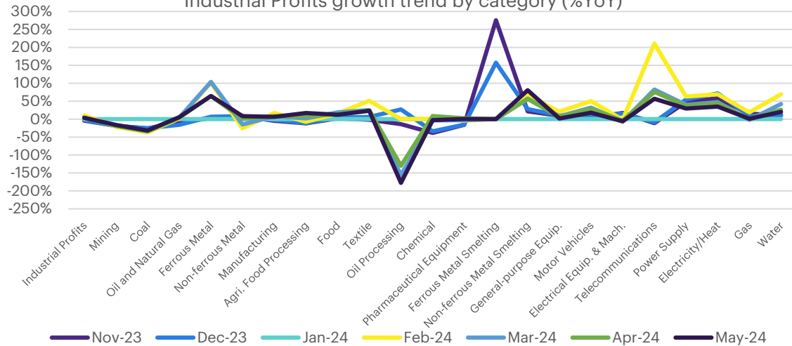
Industrial Profits growth trend by category (%YoY)
