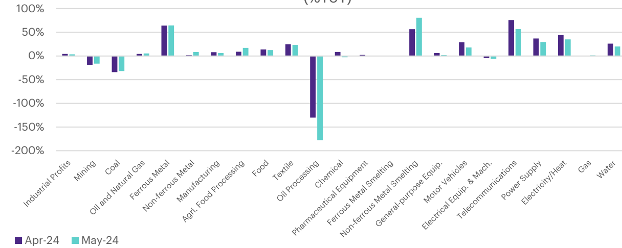
Industrial Profits growth trend by category (%YoY)
