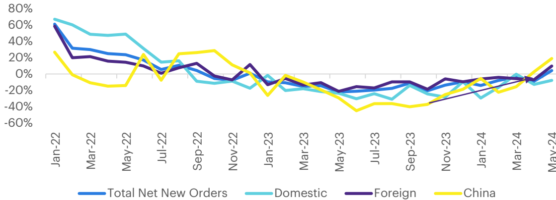
Japan machine-tool order growth - %Chg YoY
