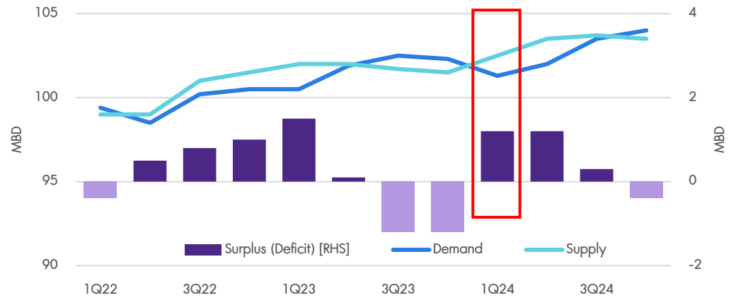
Figure 7: Oil Market Possibly Turning Deficit If Voluntarily Cut Continues
