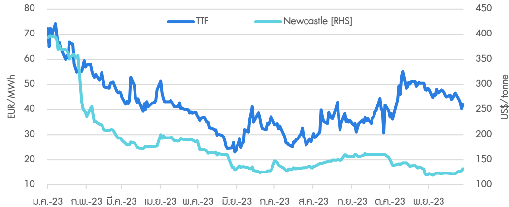
Figure 5: Declining TTF Prices Suppressing Coal Price Upside
