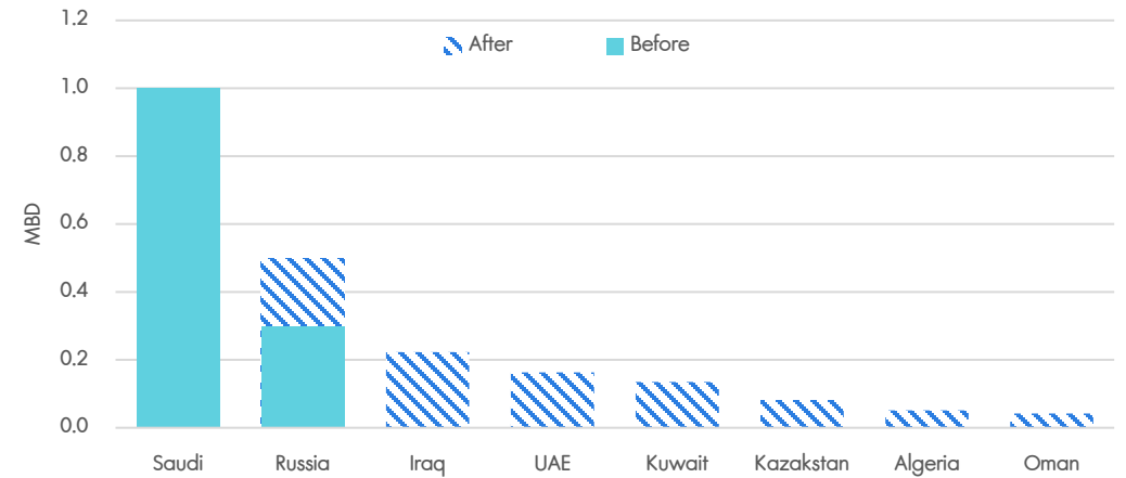
Figure 8: Saudi and Russia Oil Output Before New Voluntarily Cut
