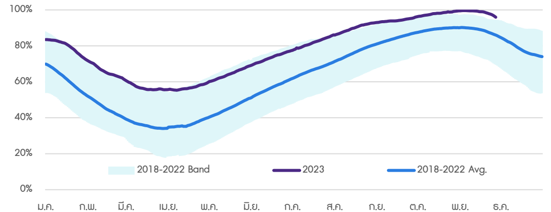
Figure 4: EU Natural Gas Level Remained High and Above 5-yr Band
